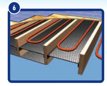
Radiant Floor / Plancher chauffant / Piso radiante
